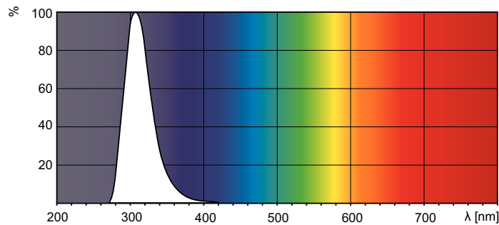
XDPO_XUMTLRS_12-Spectral power distribution Colour
