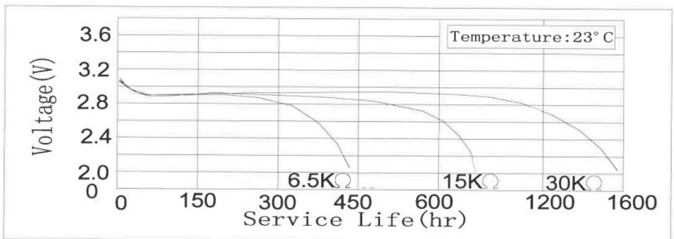
Chart 1. Discharge diagram
