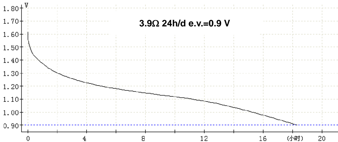
Chart 1. Discharge diagram
