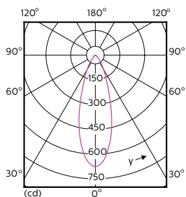
MASTER LEDspot ExpertColor MV 35W GU10 930 36D
